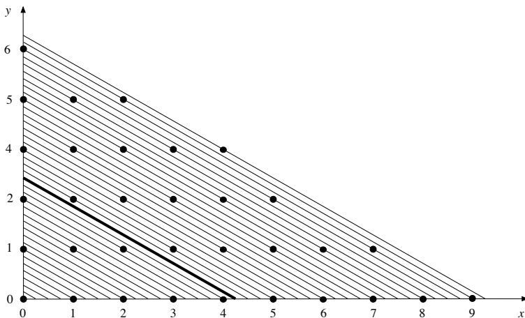
FIGURE 1. 4x + 7y = k , k = 1, 2, \dots
